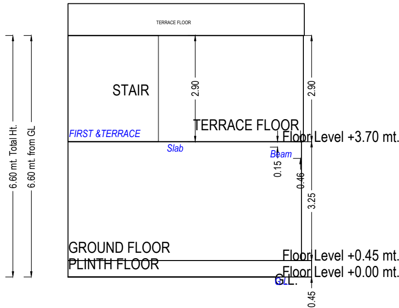
SECTION
