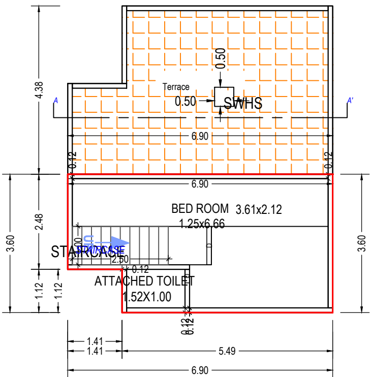
FIRST & TERRACE FLOOR PLAN TERRACE FLOOR PLAN (Proposed) (SCALE 1:100)
