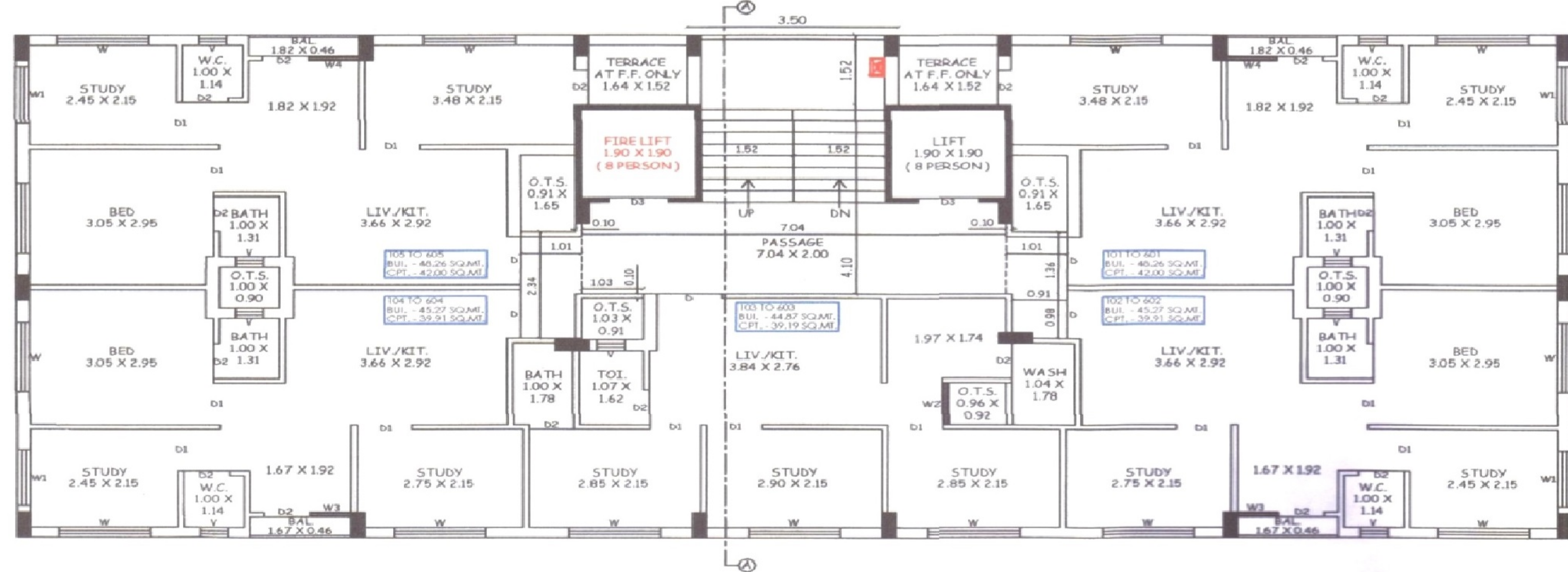
FIRST TO SIXTH FLOOR PLAN SCALE - 1:100
