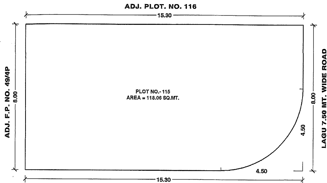
ORIGINAL PLOT PLAN SCALE :- 1:100
