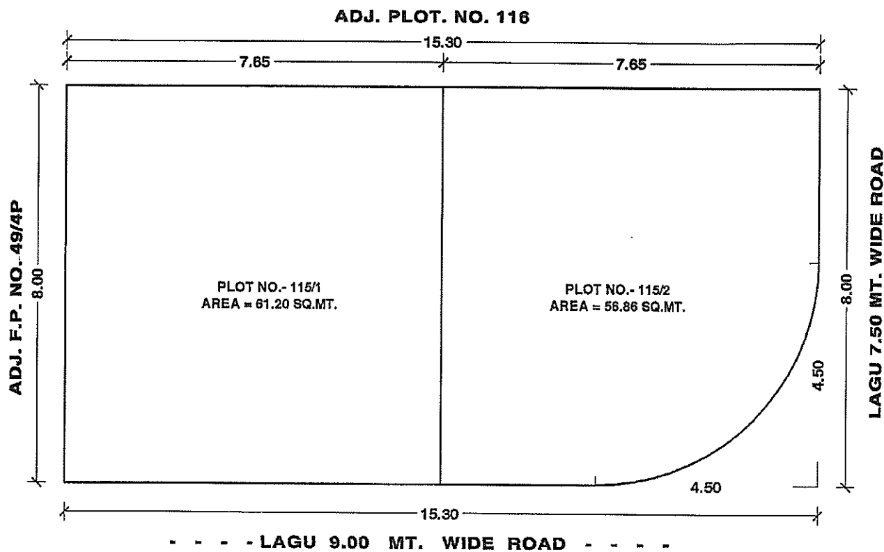
SUB PLOT PLAN SCALE :- 1:100
