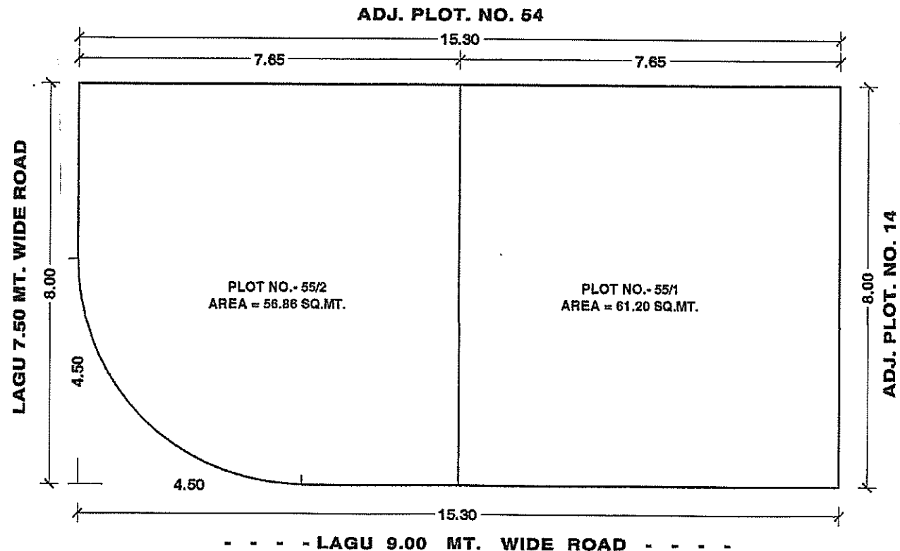
SUB PLOT PLAN
