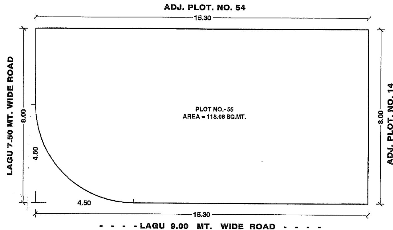
ORIGINAL PLOT PLAN
