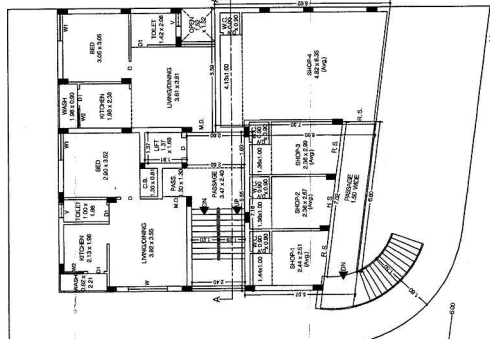
FIRST FLOOR PLAN SCALE: 1/8" = 1'-0"
