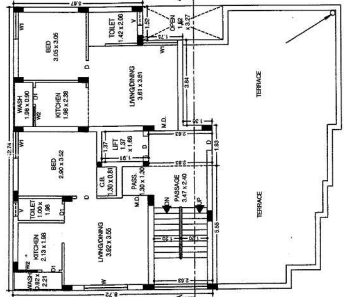
FIFTH FLOOR PLAN SCALE: 1/8" = 1'-0"
