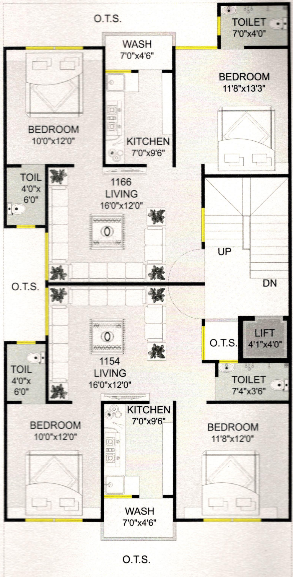
TYPICAL 1 st TO 5 th FLOOR PLAN
