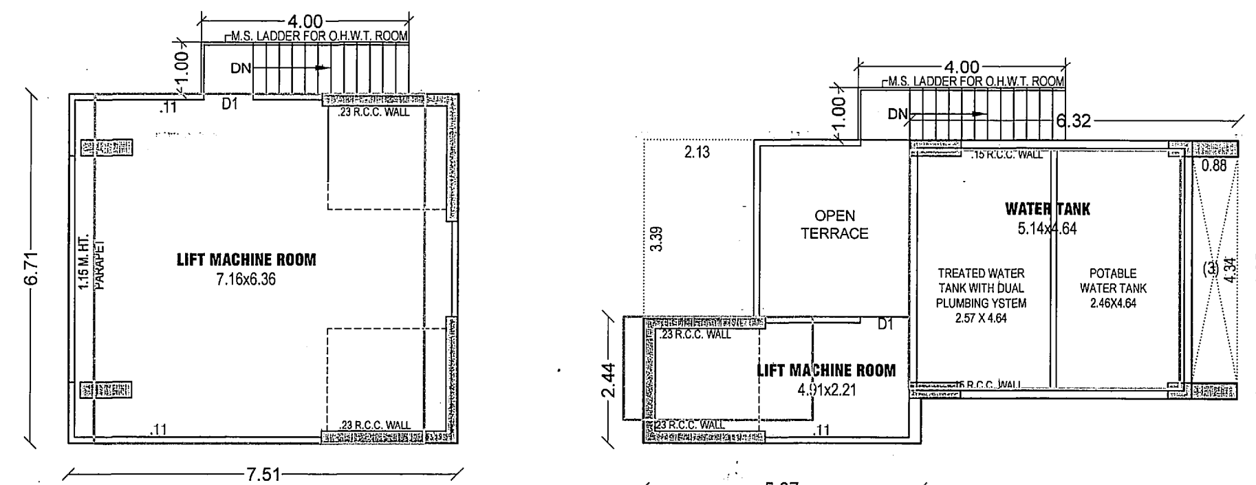
WATER TANL+ MACHINE ROOM PLAN
