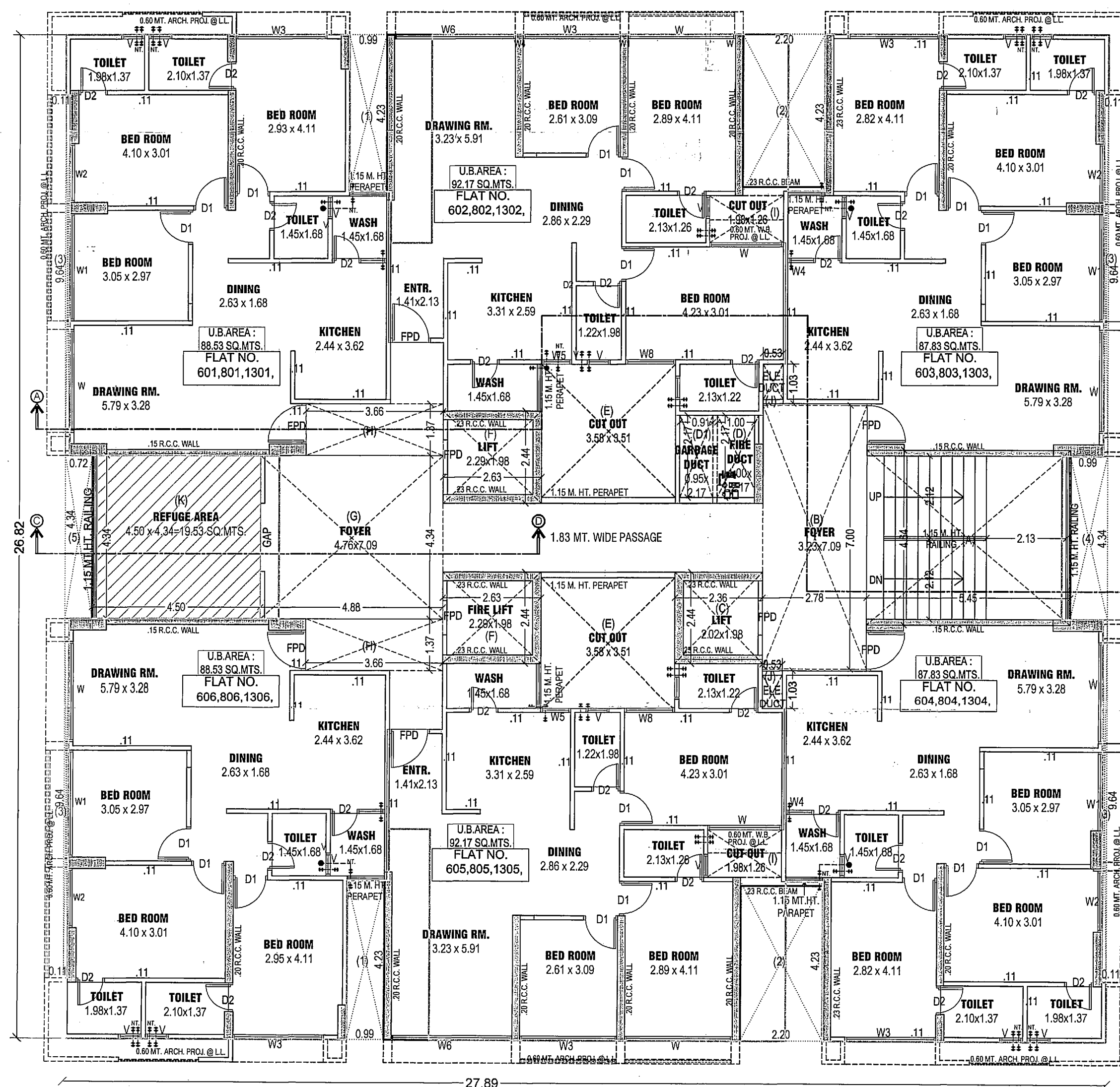
6TH, 8TH &amp; 13TH FLOOR PLAN
