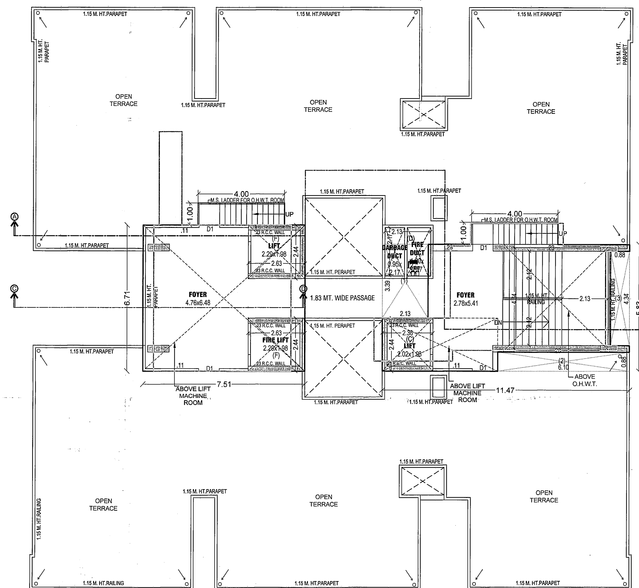
OPEN TERRACE + STAIR CABIN PLAN
