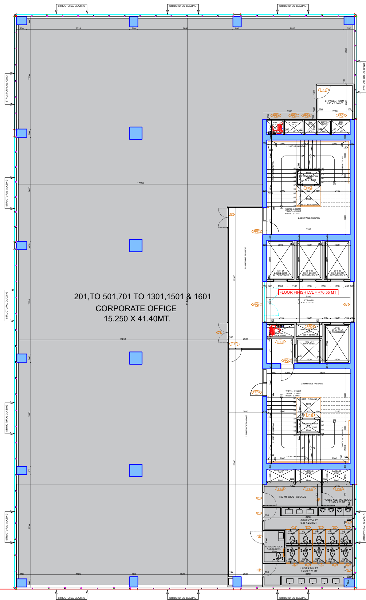
2ND TO 5TH, 7TH TO 13TH, 15TH & 16TH FLOOR PLAN
