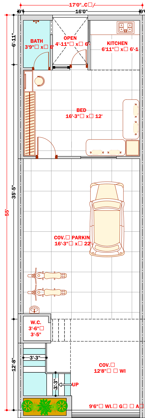
GROUND FLOOR
