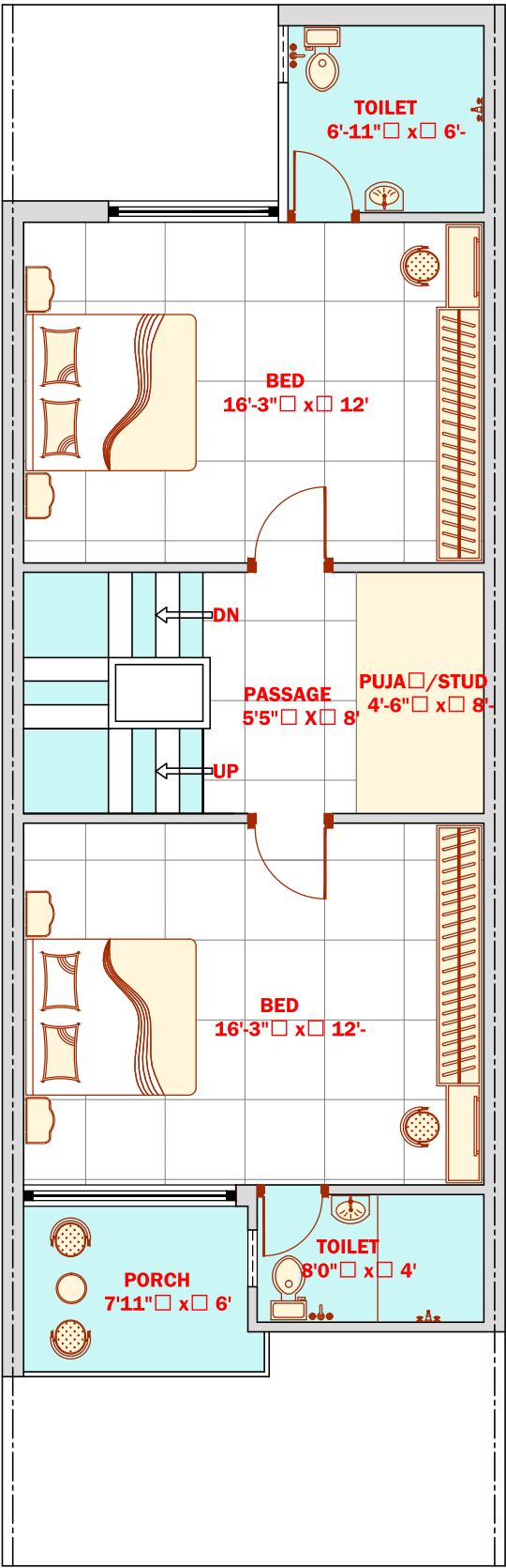
SECOUND FLOOR
