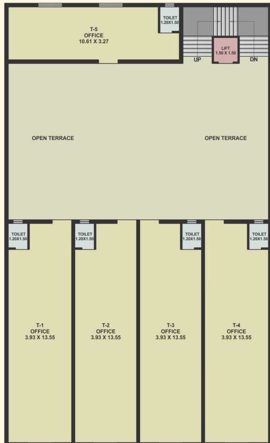
THIRD FLOOR PLAN SCALE 1.0 CM = 1.0 MT
