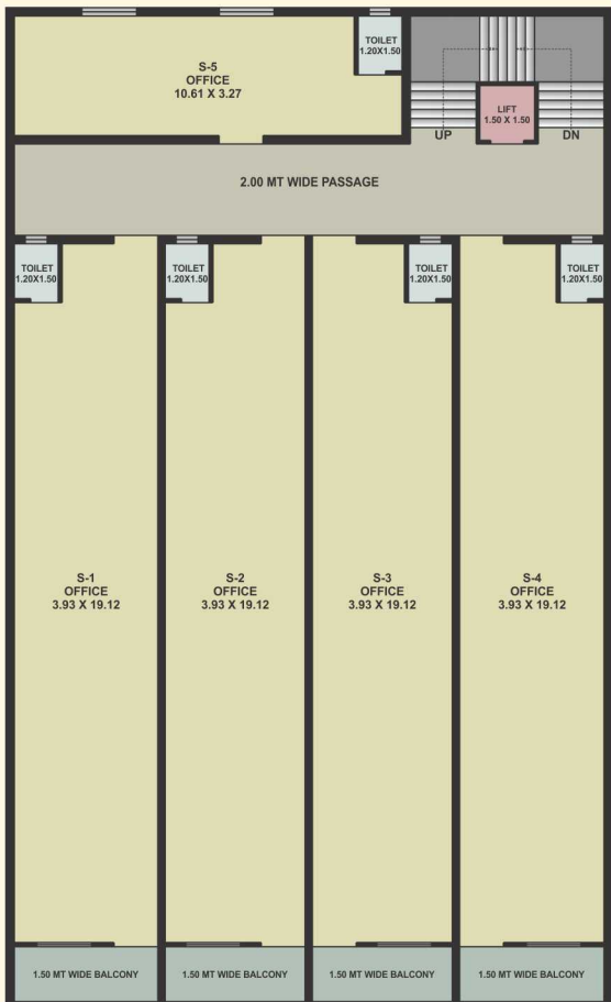
SECOND FLOOR PLAN SCALE 1.0 CM = 1.0 MT
