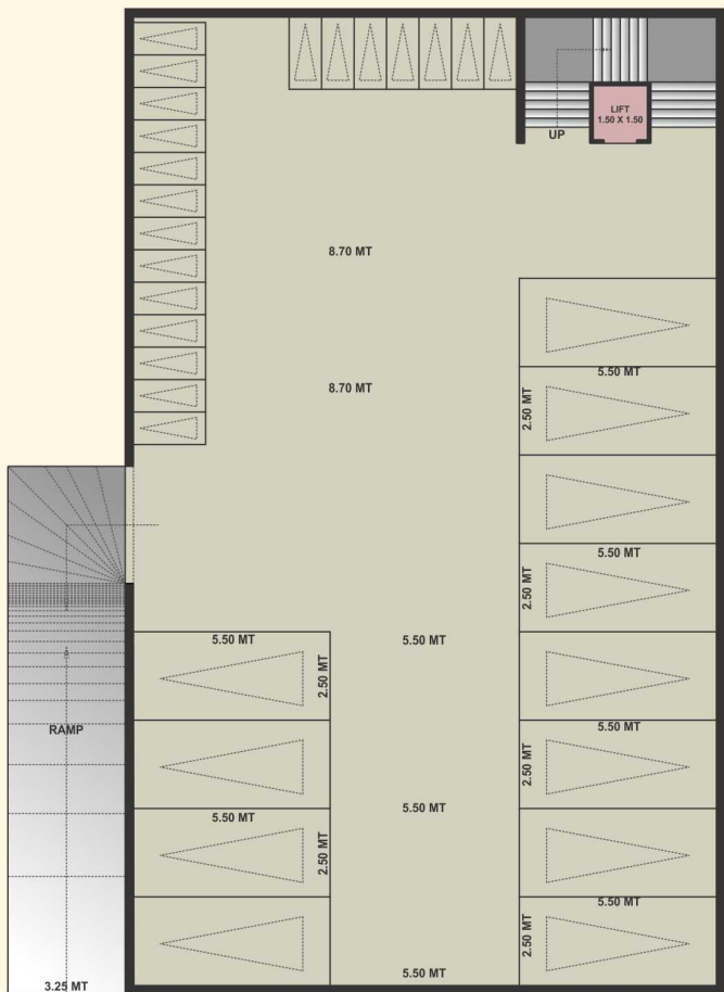
BASEMENT FLOOR PLAN SCALE 1.0 CM = 1.0 MT
