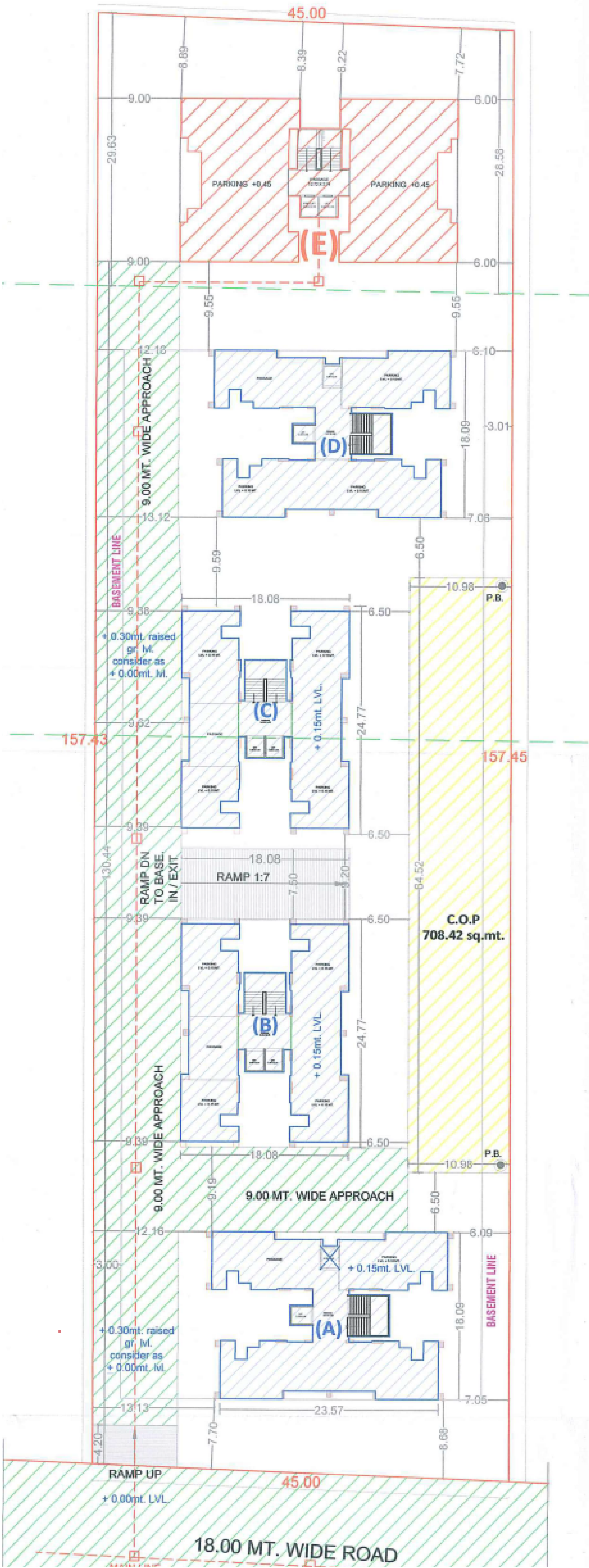
LAYOUT PLAN
