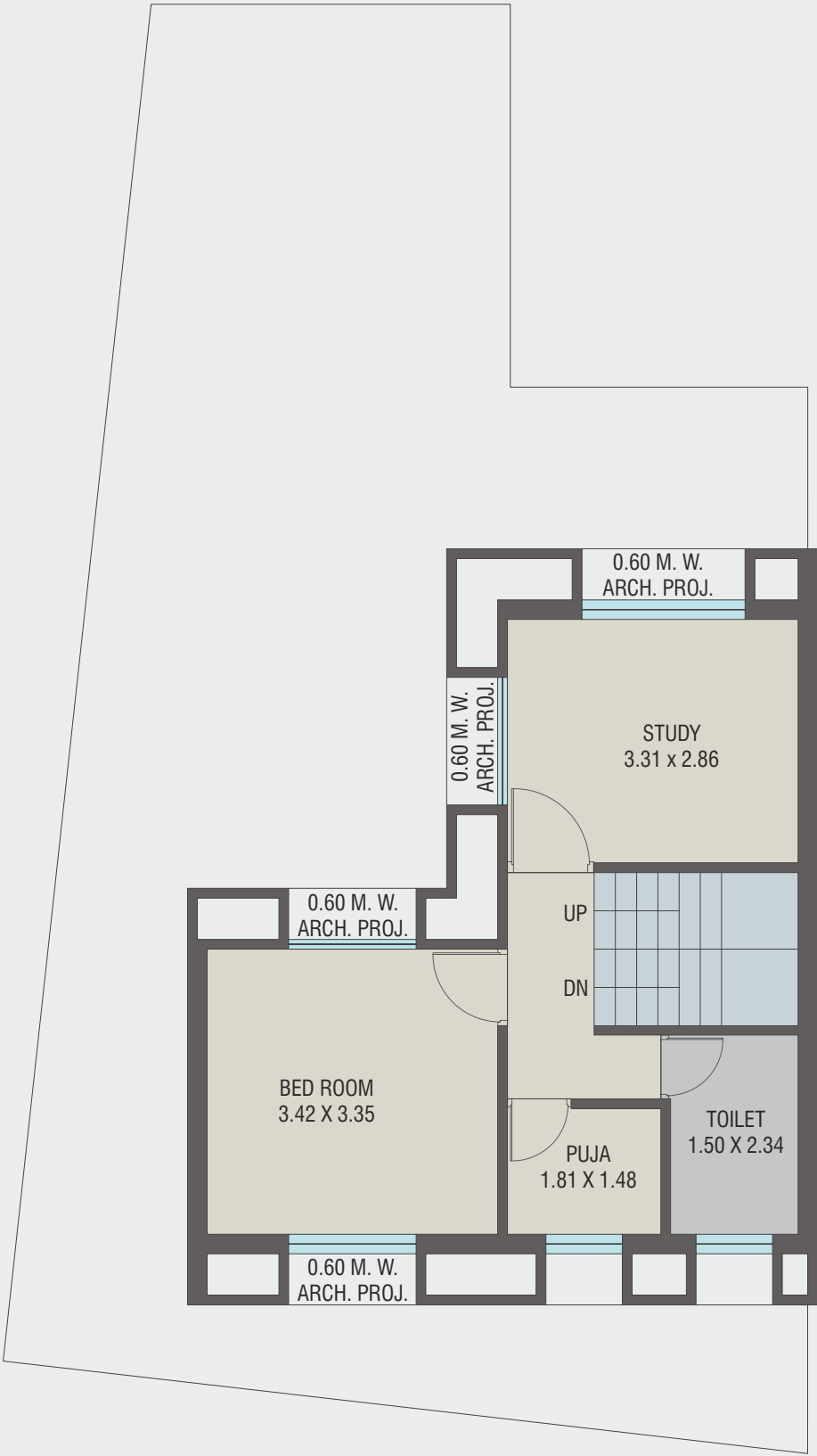
First Floor
