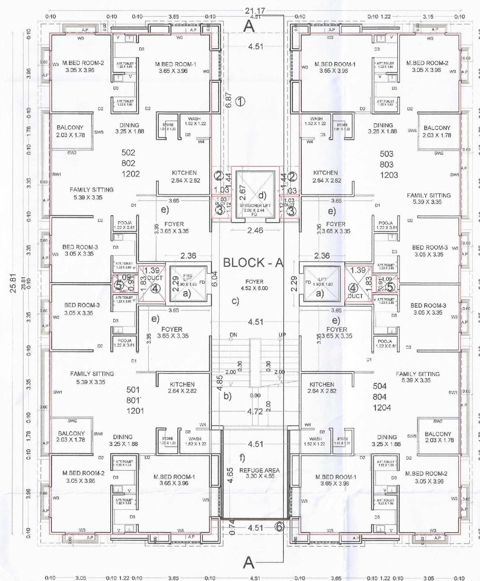
5TH, 8TH & 12TH FLOOR PLAN
