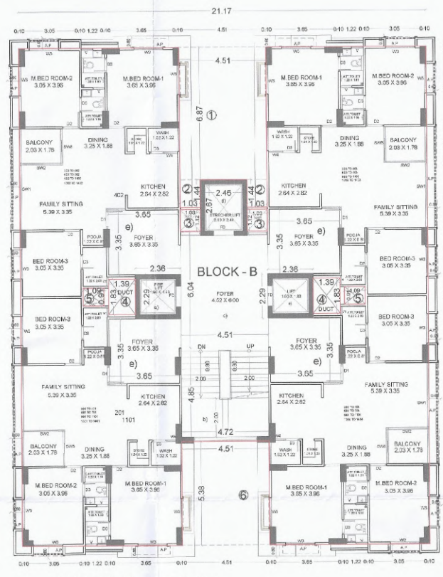
TYPICAL FLOOR PLAN (3rd FL, 4th FL, 6th FL, 7th FL, 9th FL, 10th, 11th, 13th, 14th)
