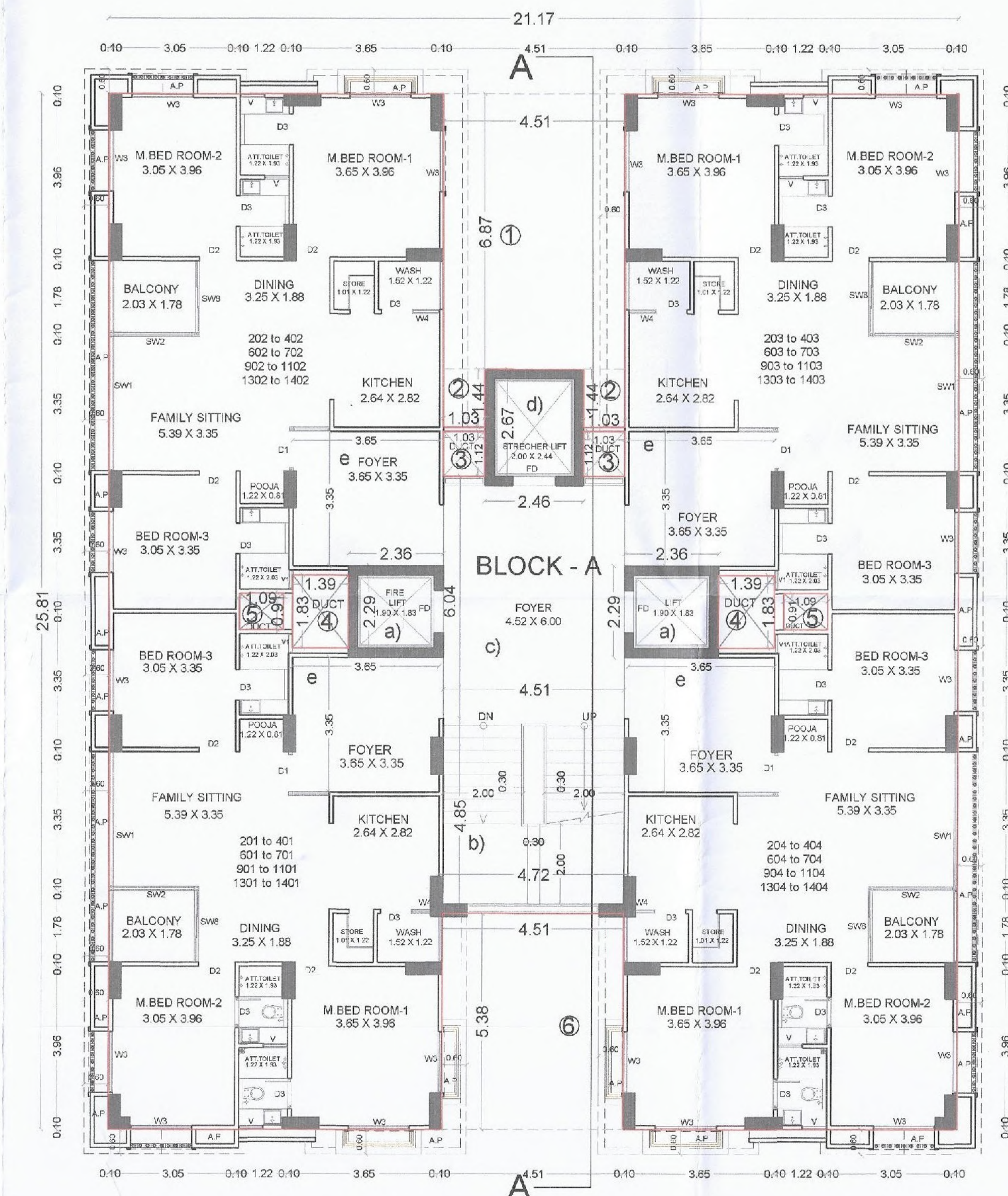
TYPICAL FLOOR PLAN (2ND FL, 3rd FL, 4th FL, 6th FL, 7th FL, 9th FL, 10th, 11th, 13th, 14th)
