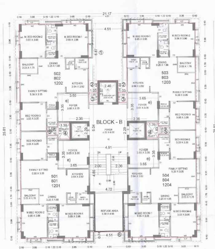
5TH, 8TH &amp; 12TH FLOOR PLAN
