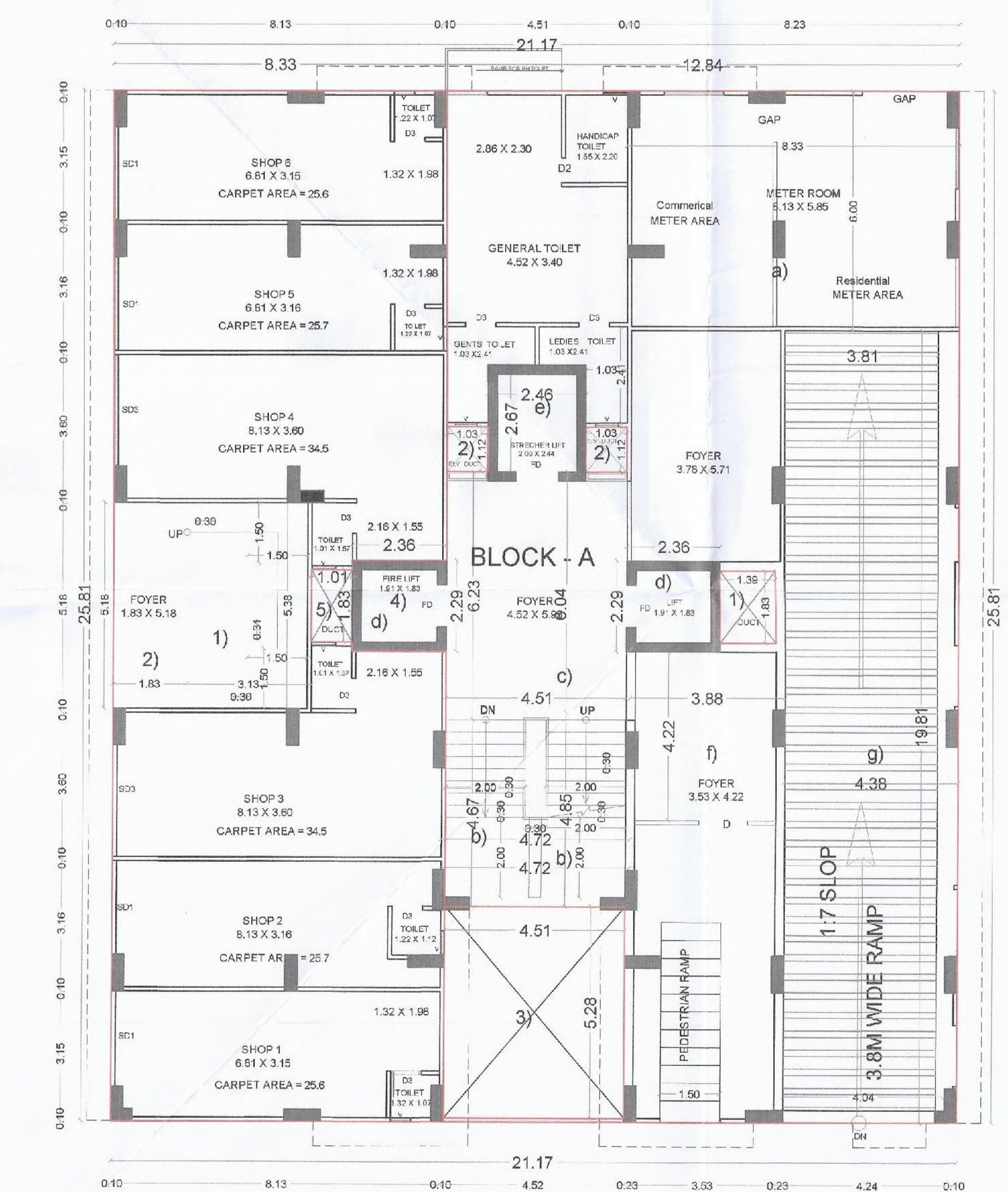
GROUND FLOOR(hp)
