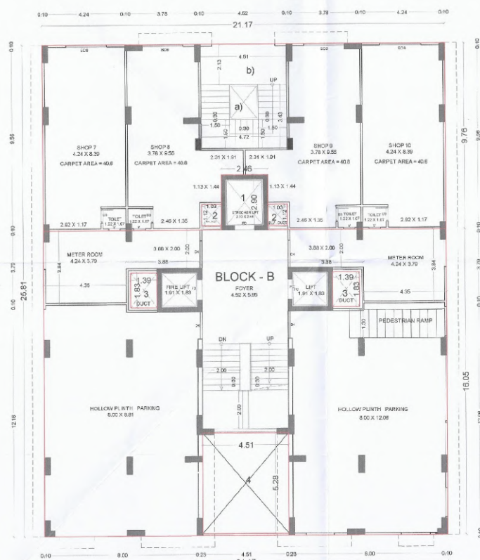
GROUND FLOOR(h.p)
