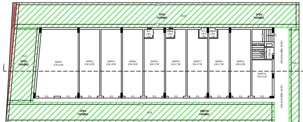
G.F. PLAN SCALE 1:100
