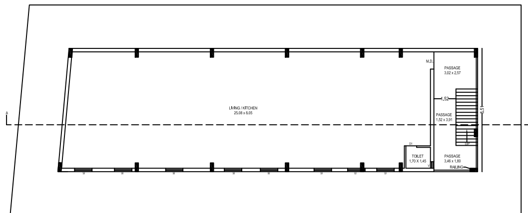
S.F. PLAN SCALE 1:100
