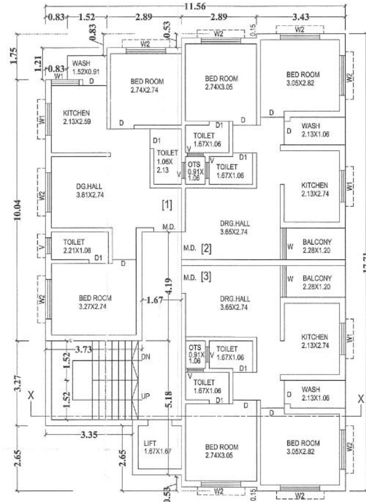
1st TO 5th FLOOR PLAN
