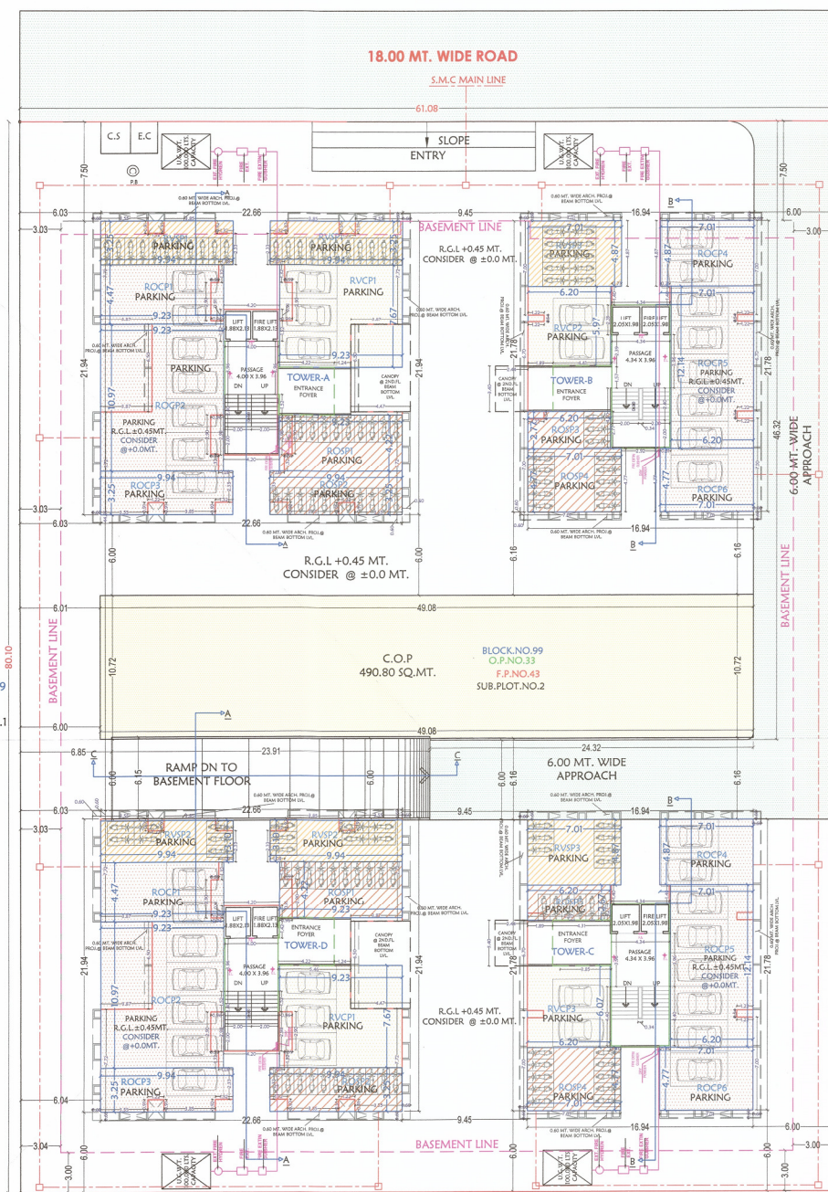
GROUND FLOOR PARKING PLAN R.G.L. +0.45 MT. CONSIDER @ +0.0 MT. SCALE - 1 CM. = 2.00 MT.
