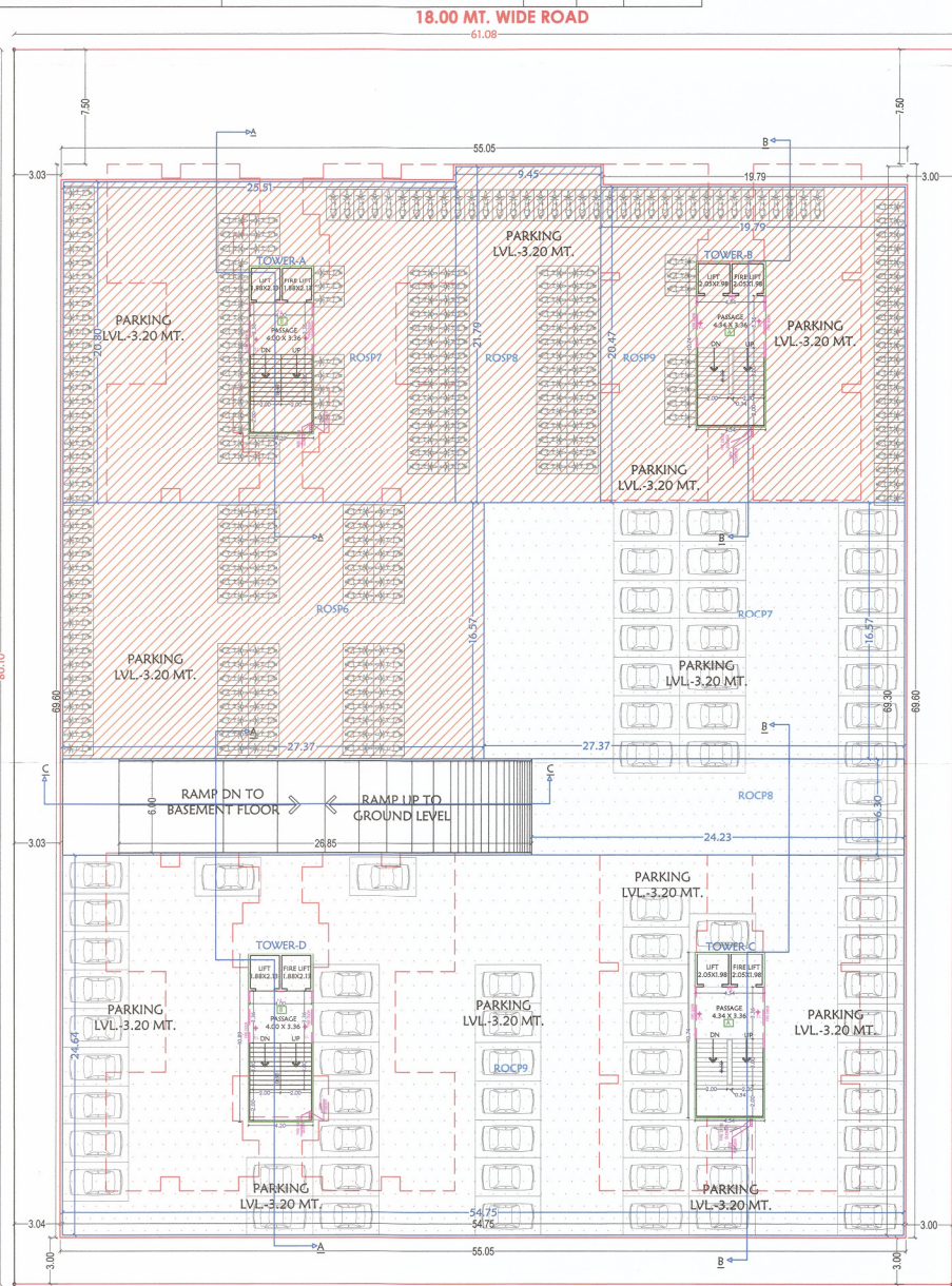
BASEMENT FLOOR PARKING PLAN LVL. -3.20 MT. SCALE - 1 CM. = 2.00 MT.
