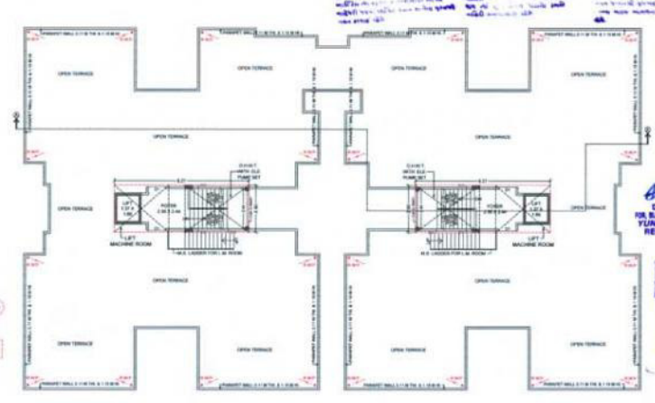
OPEN TERRACE & STAR CABIN, LIFT M.R. PLAN
