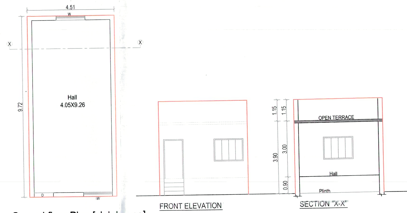
Ground floor Plan [club house] BUILT UP AREA : 43.83 sq.mt.
