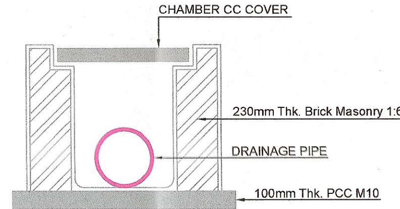
TYPICAL CROSS SECTION OF CHAMBER
