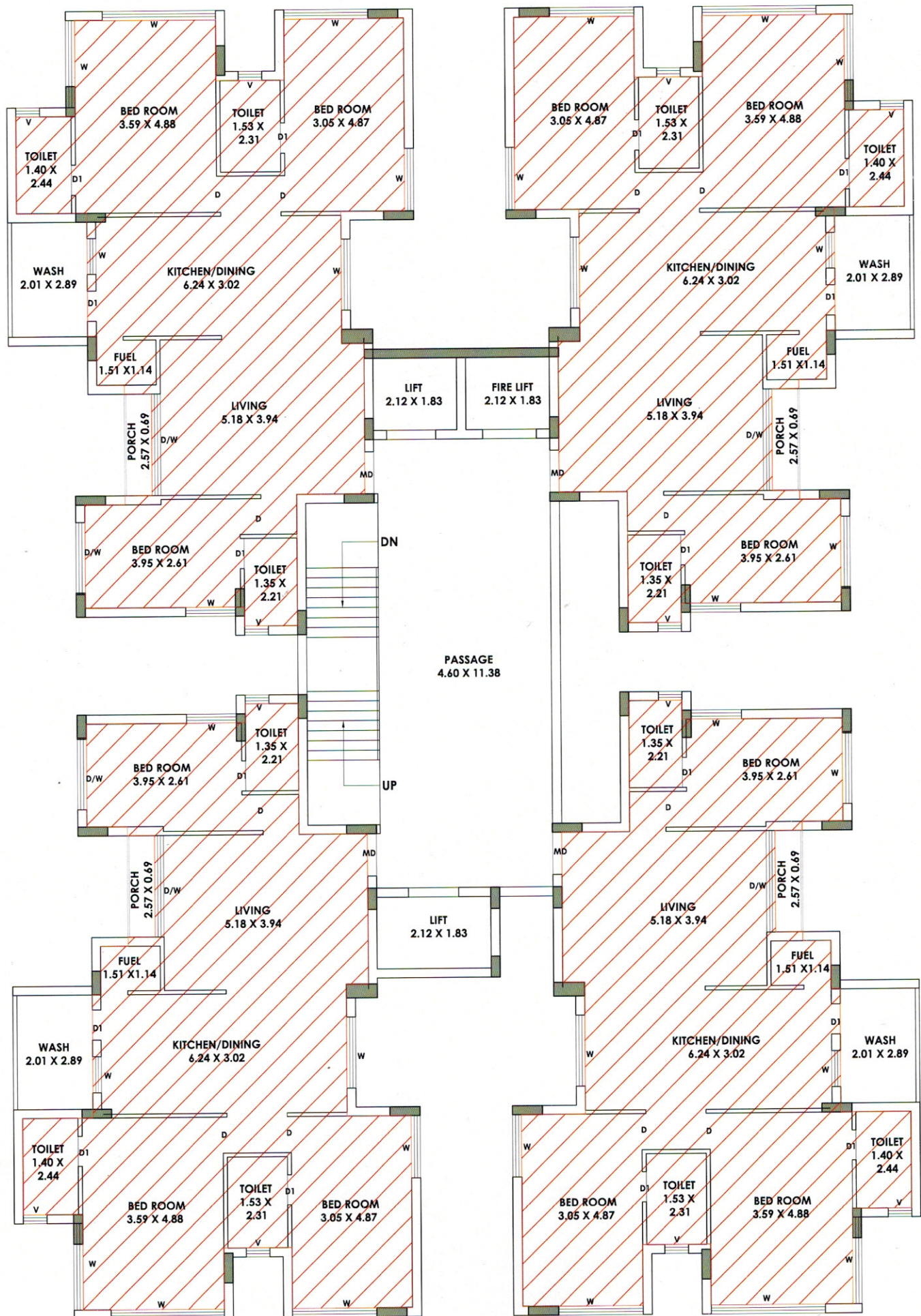
1ST TO 8TH FLOOR PLAN
