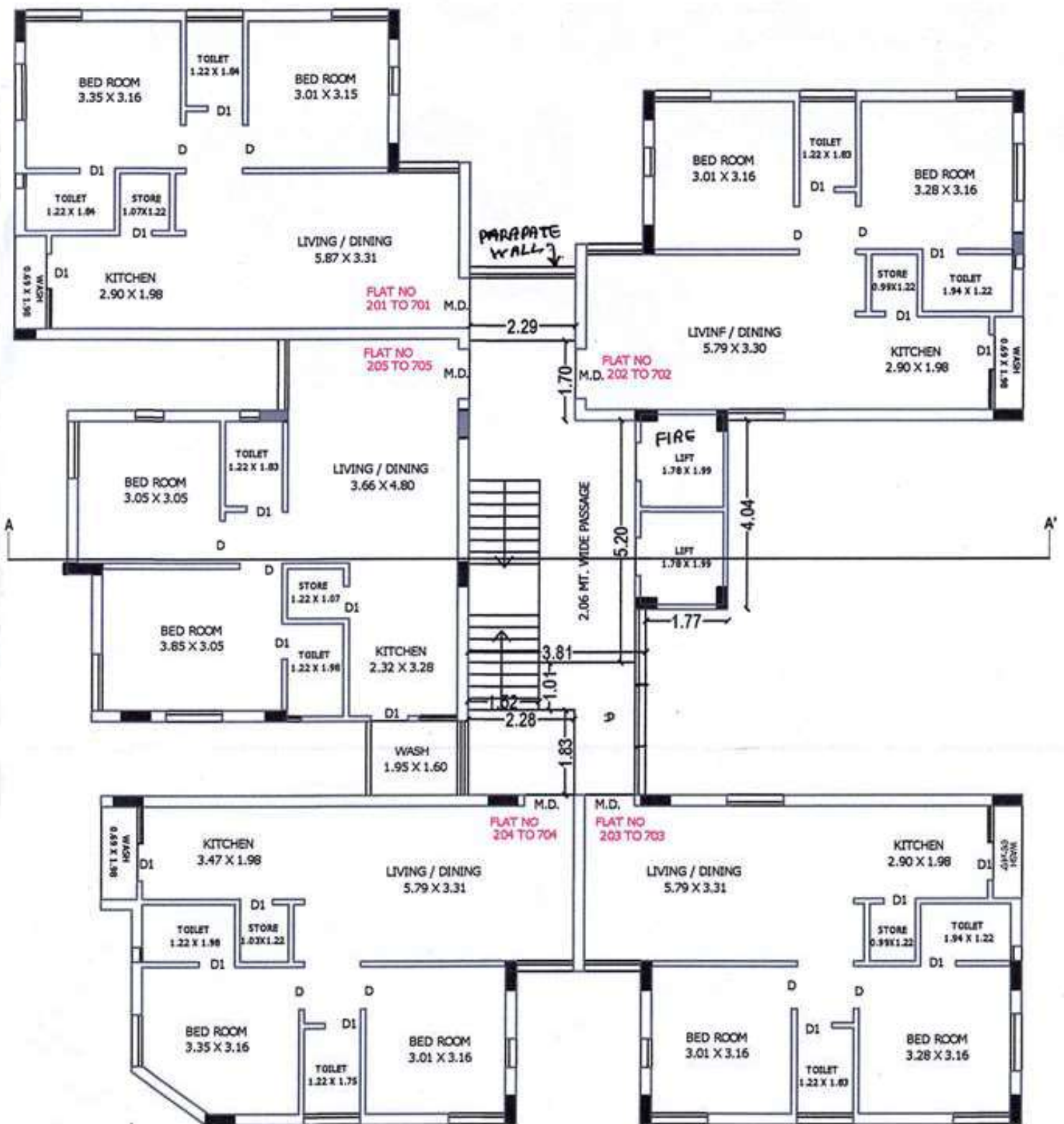
2ND TO 7TH FLOOR PLAN
