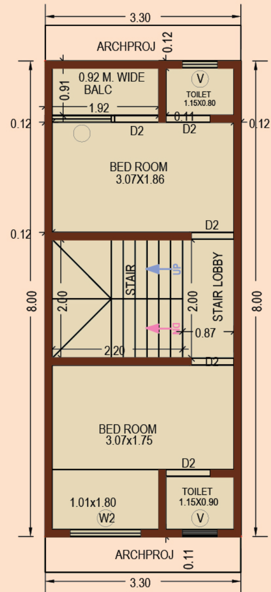
FIRST FLOOR PLAN (E - 6 Unit)
