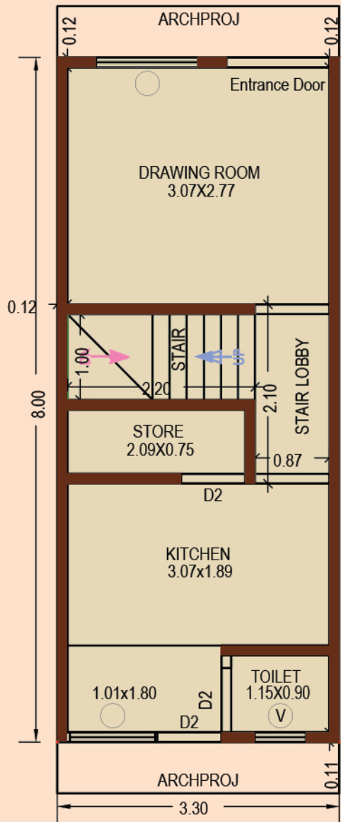
GROUND FLOOR PLAN (E - 6 Unit)
