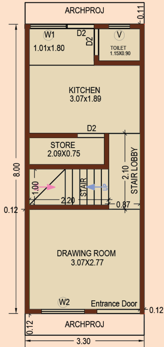
GROUND FLOOR PLAN (C - 6 Unit)
