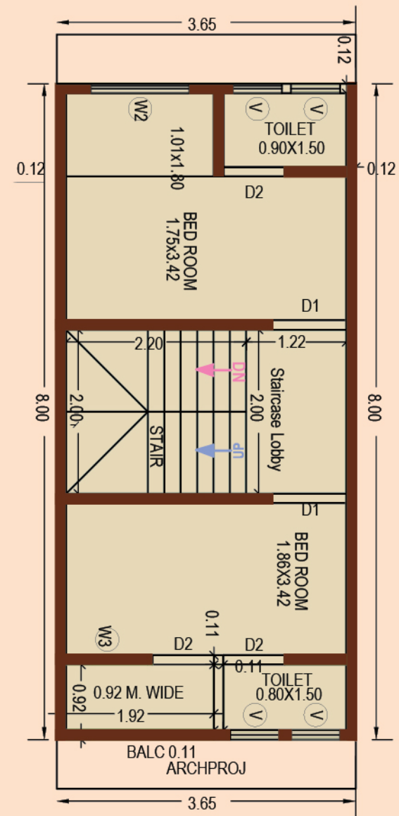
FIRST FLOOR PLAN (B - 9 Unit)
