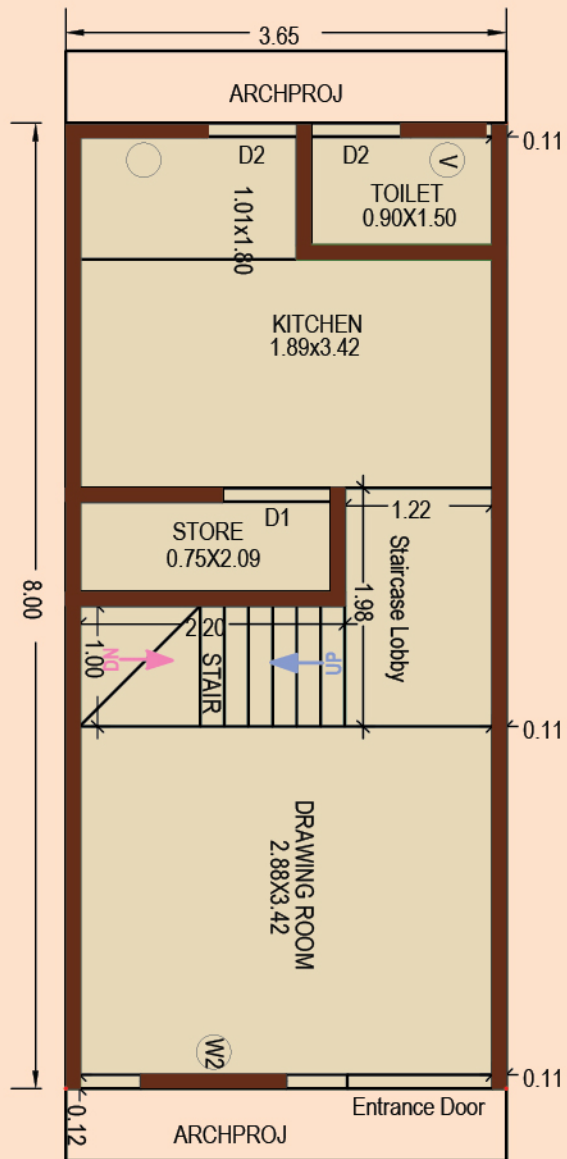
GROUND FLOOR PLAN (B - 9 Unit)
