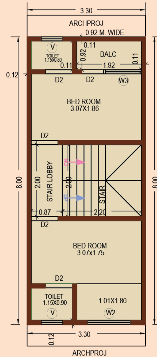
FIRST FLOOR PLAN (F - 6 Unit)
