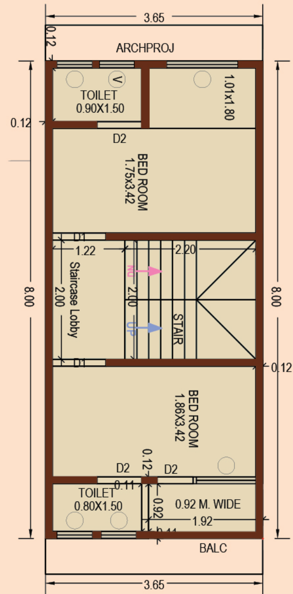
FIRST FLOOR PLAN (A - 8 Unit)
