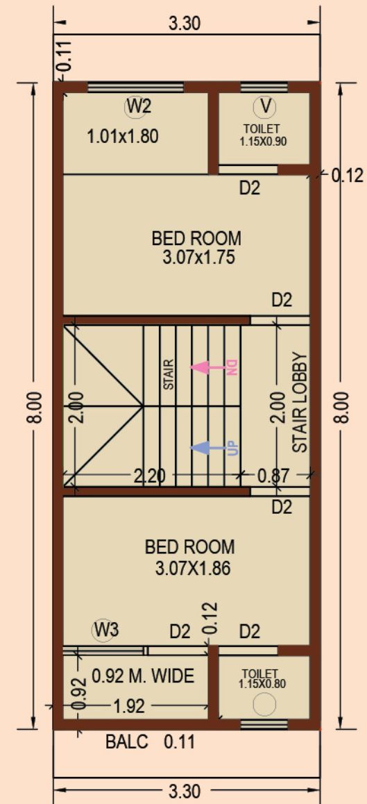
FIRST FLOOR PLAN (C - 6 Unit)
