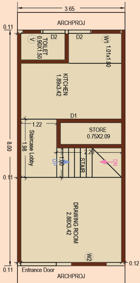
GROUND FLOOR PLAN (A - 8 Unit)
