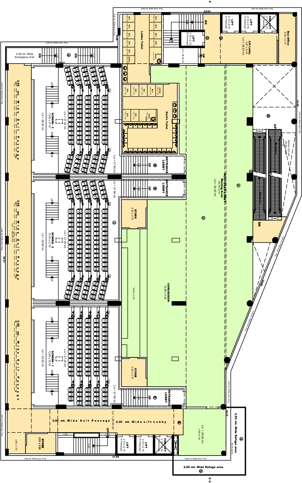
LOWER MULTIPLEX FLOOR PLAN ( 5th.Floor Lvl. + 26.00 mt)
