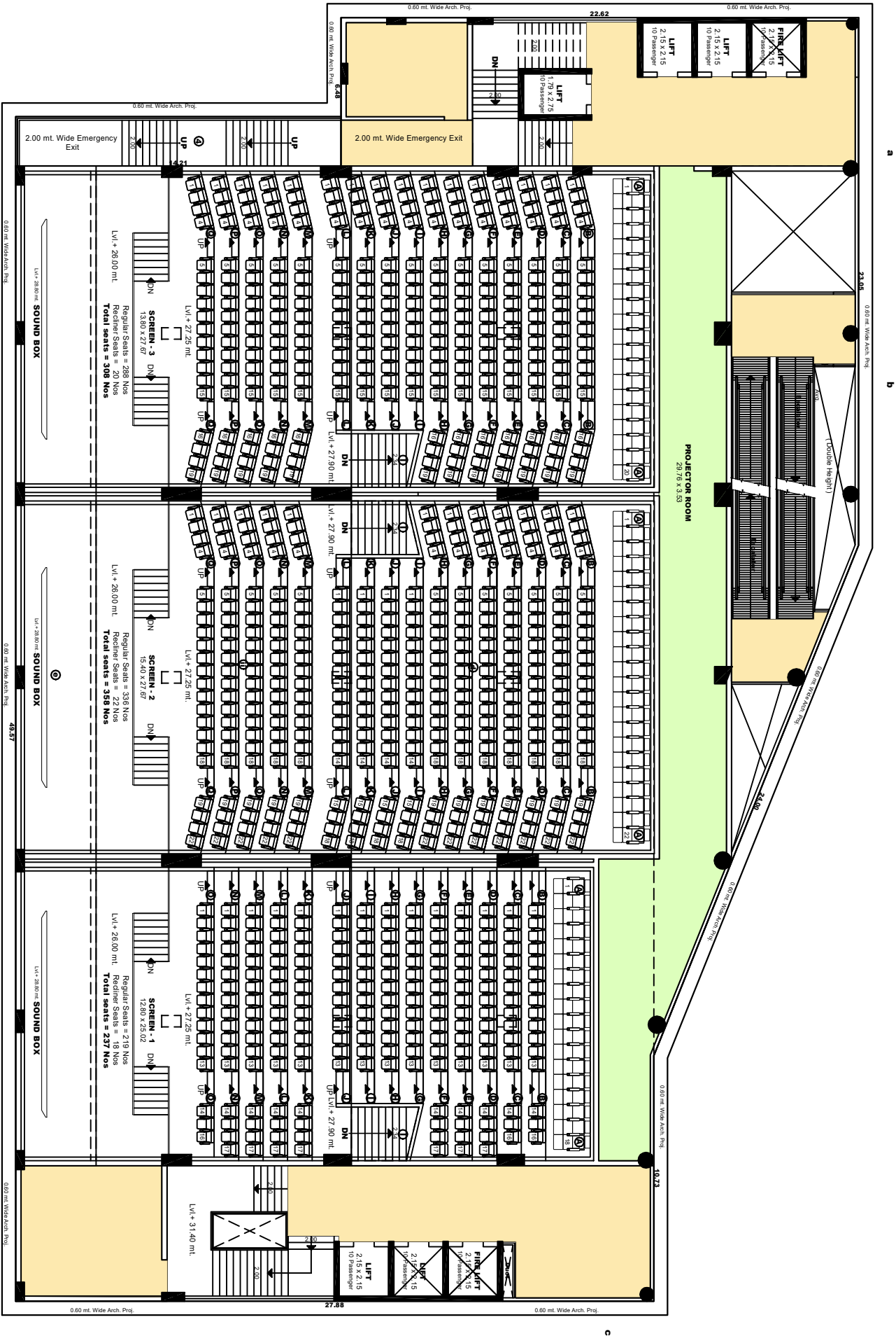
UPPER MULTIPLEX FLOOR PLAN ( 5th.Floor Lvl. + 32.30 mt.)
