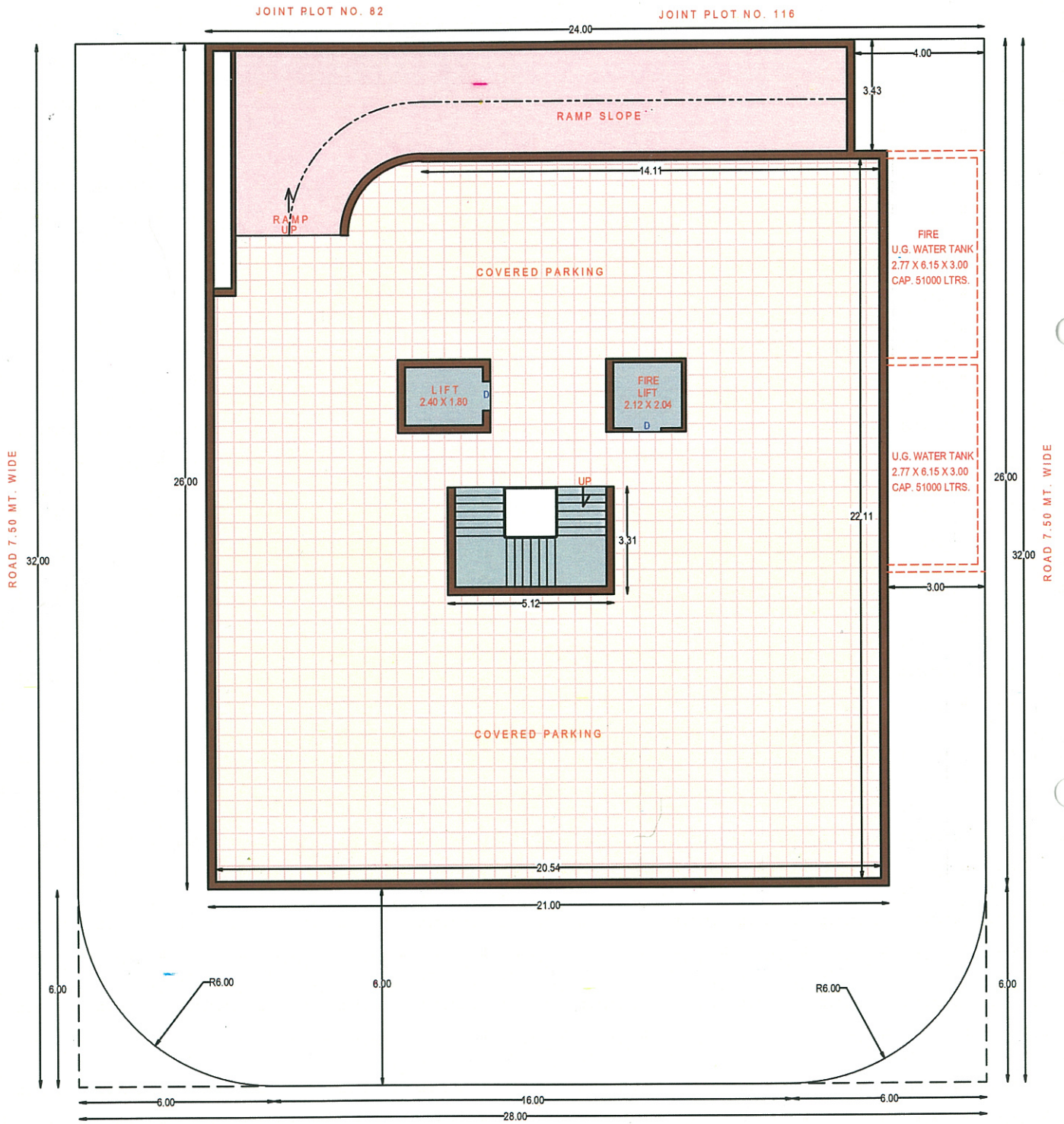
CELLER FLOOR PLAN
