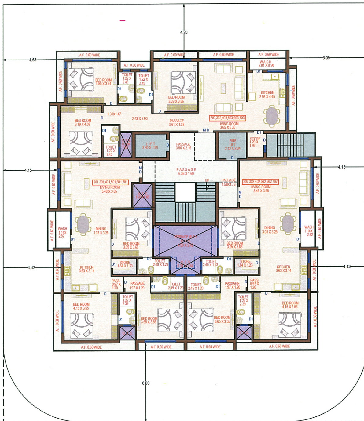
TYPICAL 2ND TO 7TH FLOOR PLAN
