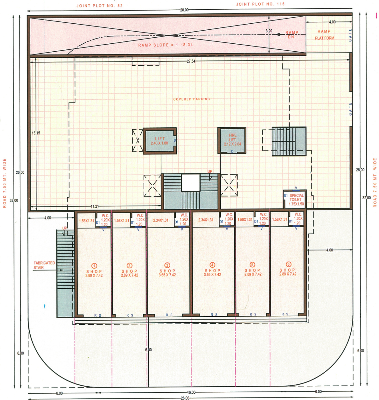
ROAD 24.00 MT. WIDE GROUND FLOOR PLAN
