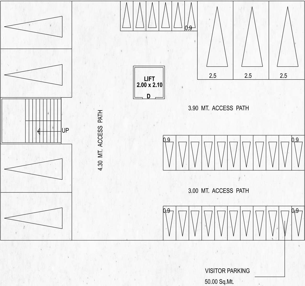
GROUND FLOOR PARKING LAY-OUT
