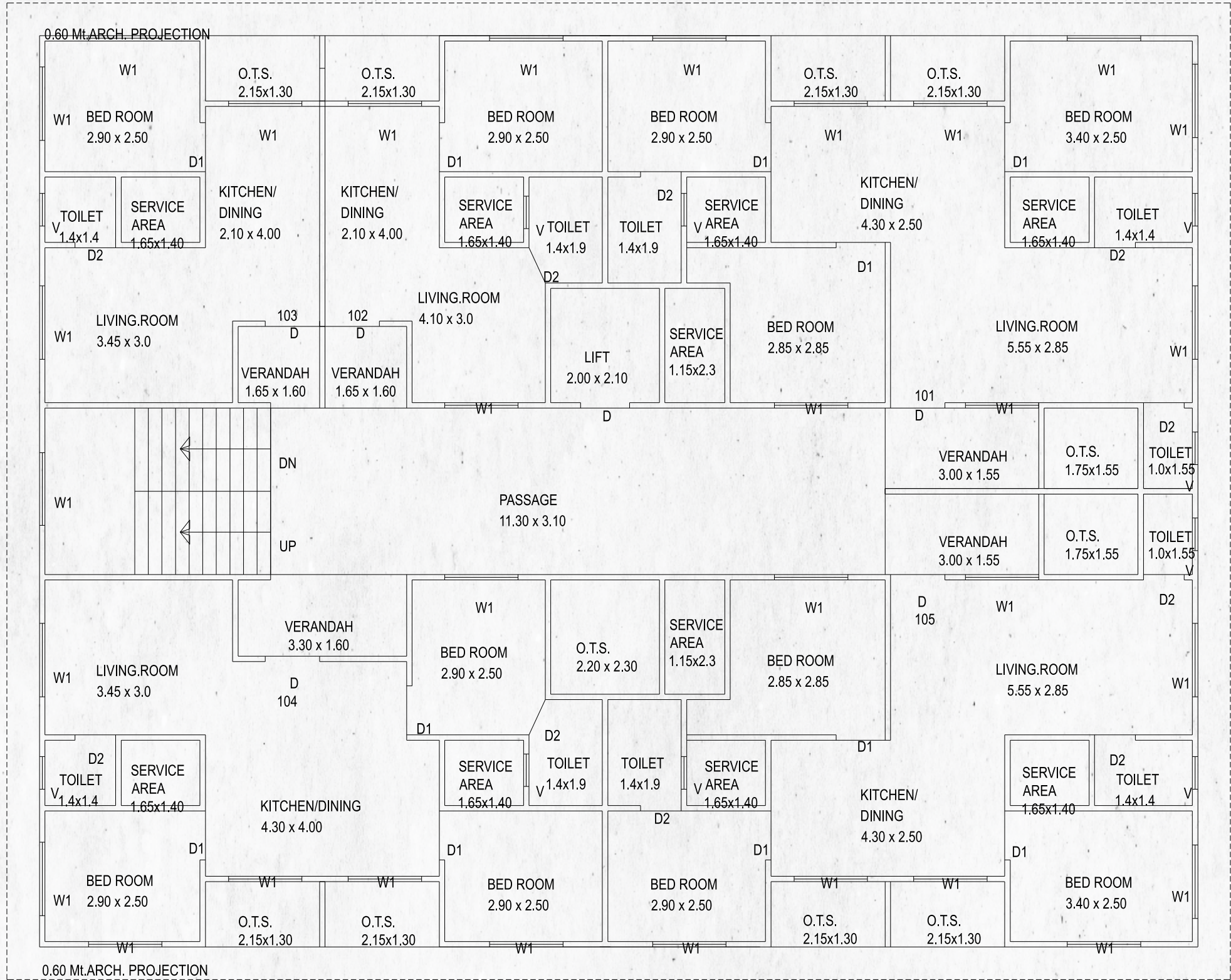
1st.FLOOR TO 5th. FLOOR PLAN
