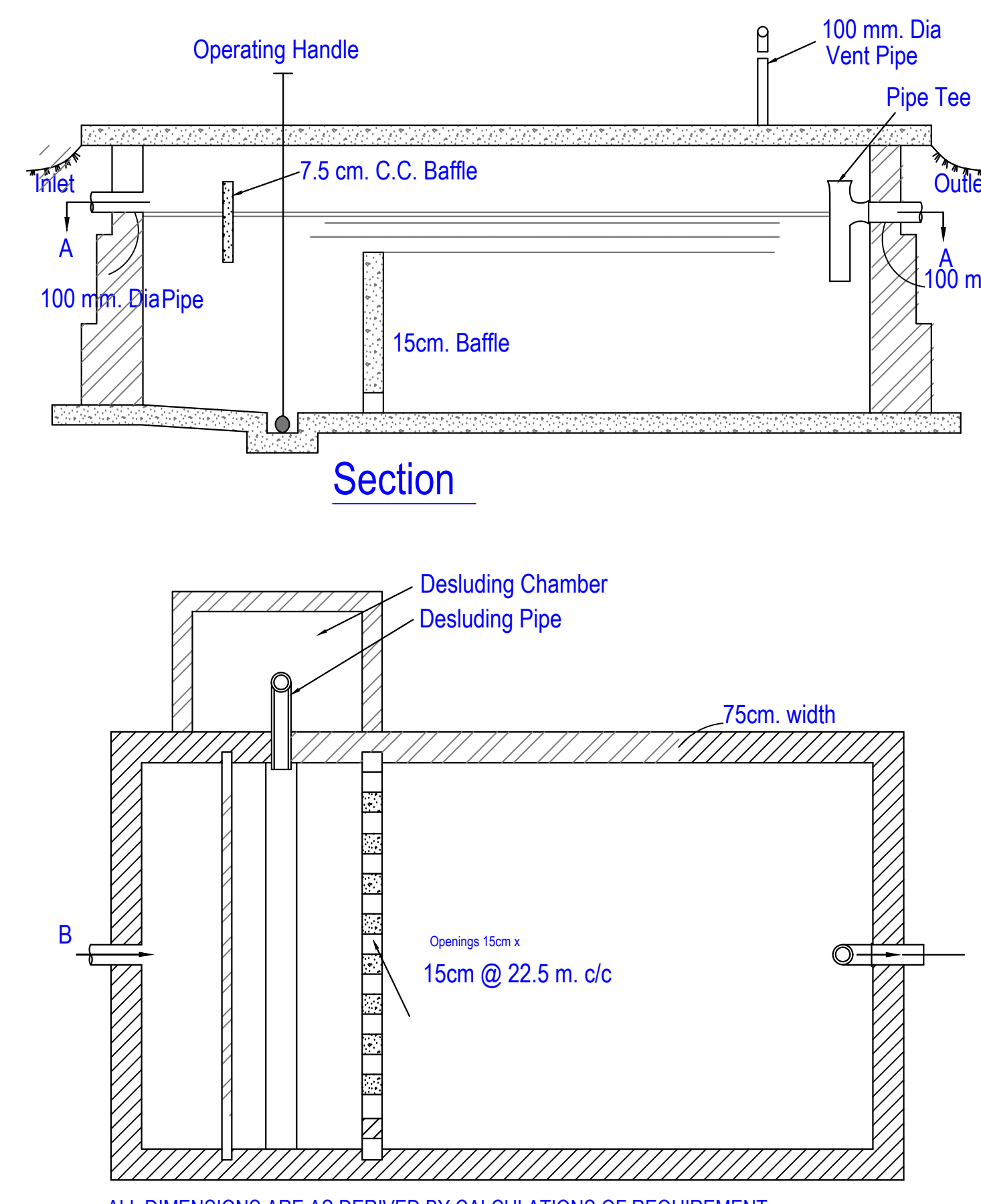
Septic Tank
