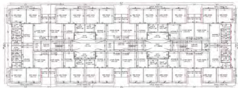
→ TYPICAL - UPPER GROUND, 1- 4 FLOOR PLAN ( SCALE 1:100 )
