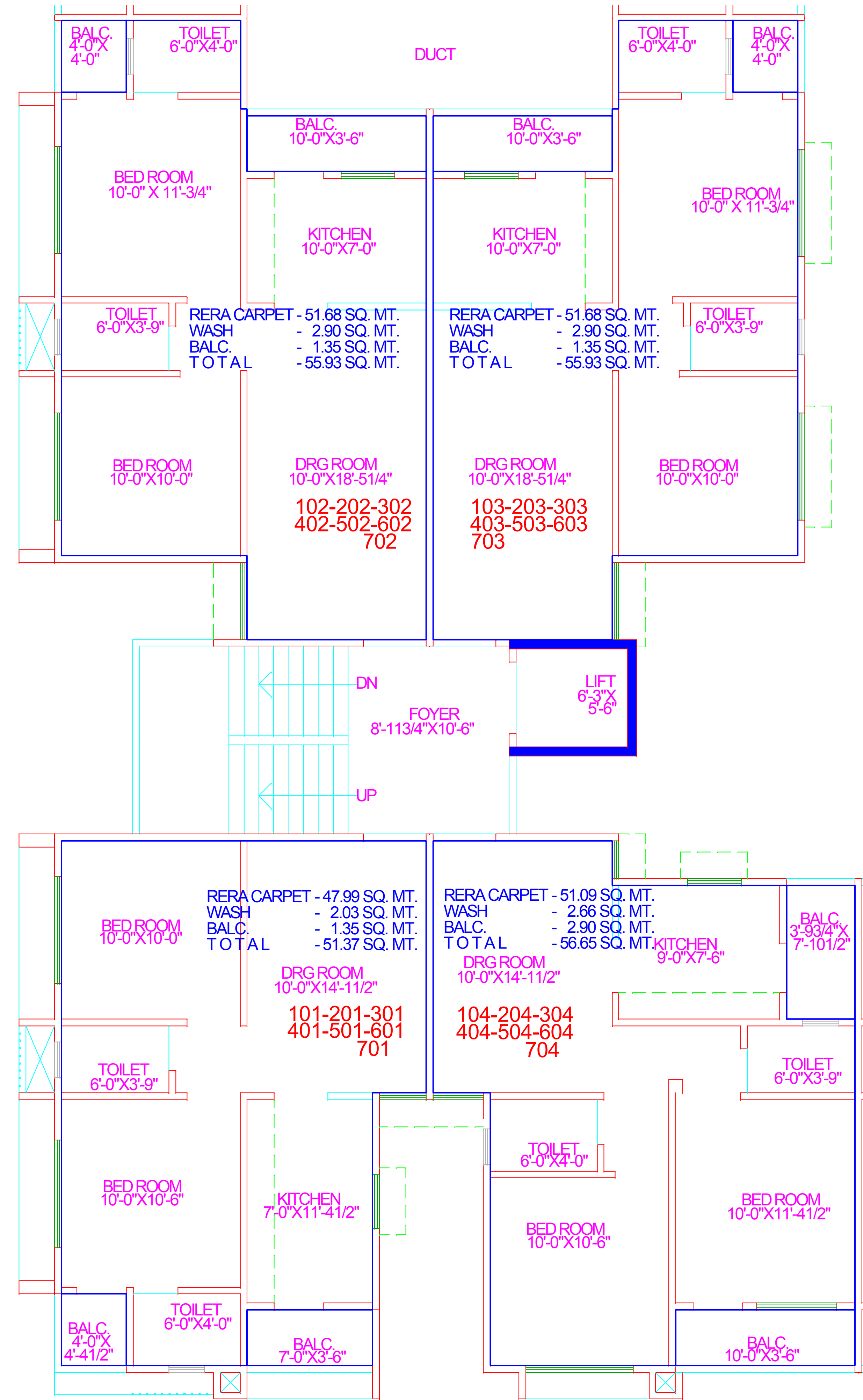
TYPICAL FLOOR PLAN (BLOCK B)
