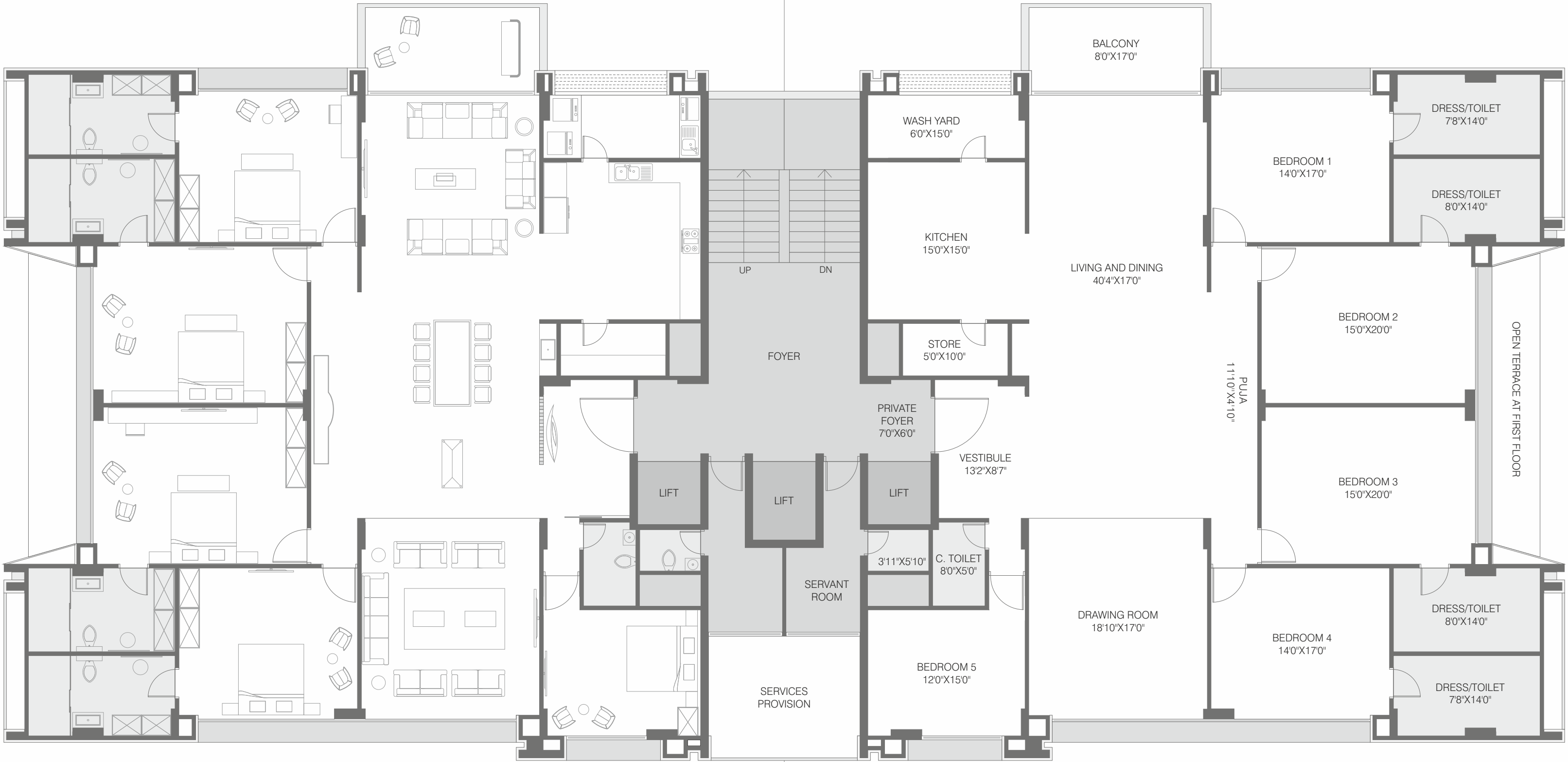
TYPICAL FLOOR
