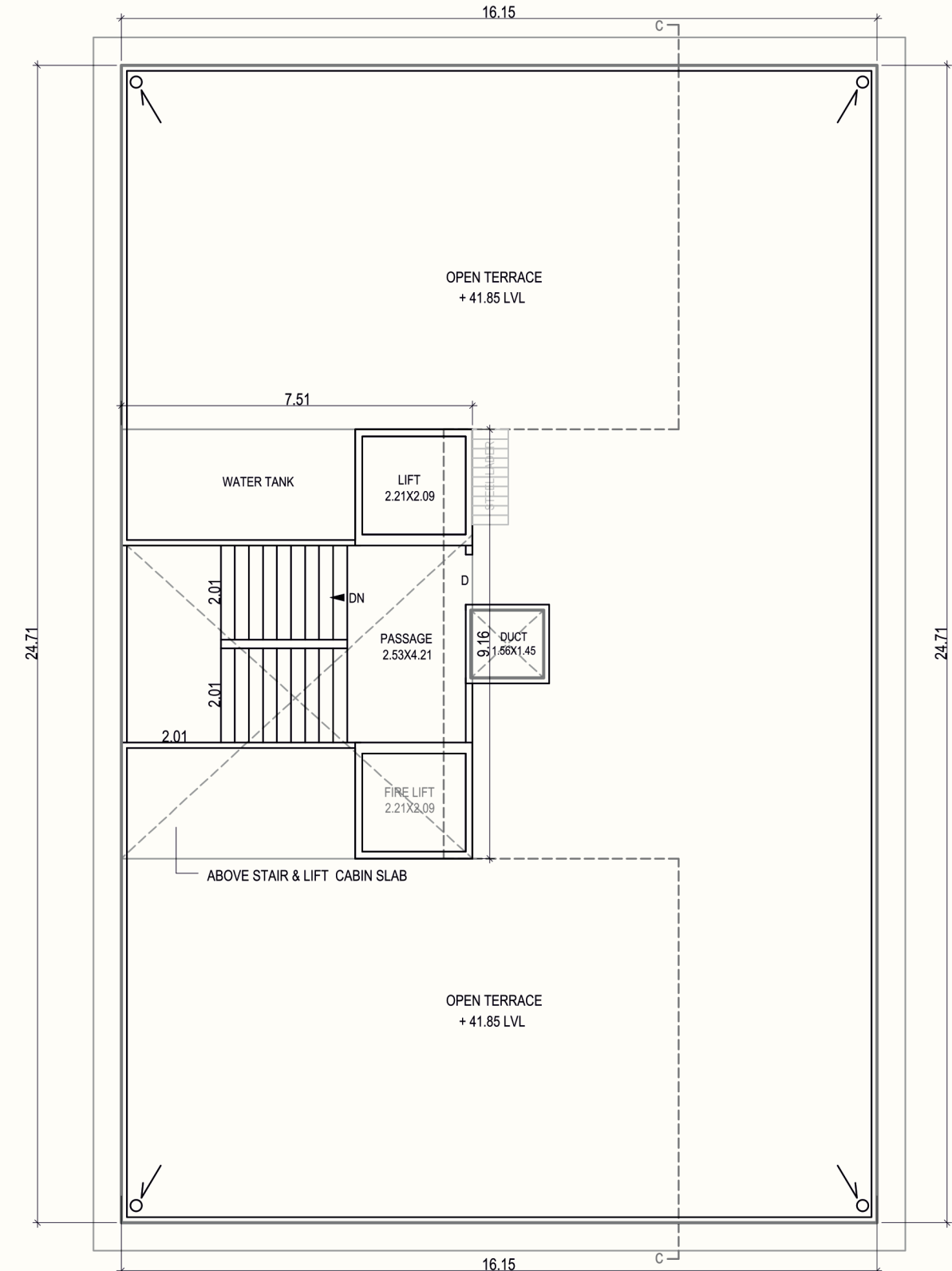
C-D-E-F BUILDING TERRACE FLOOR PLAN
