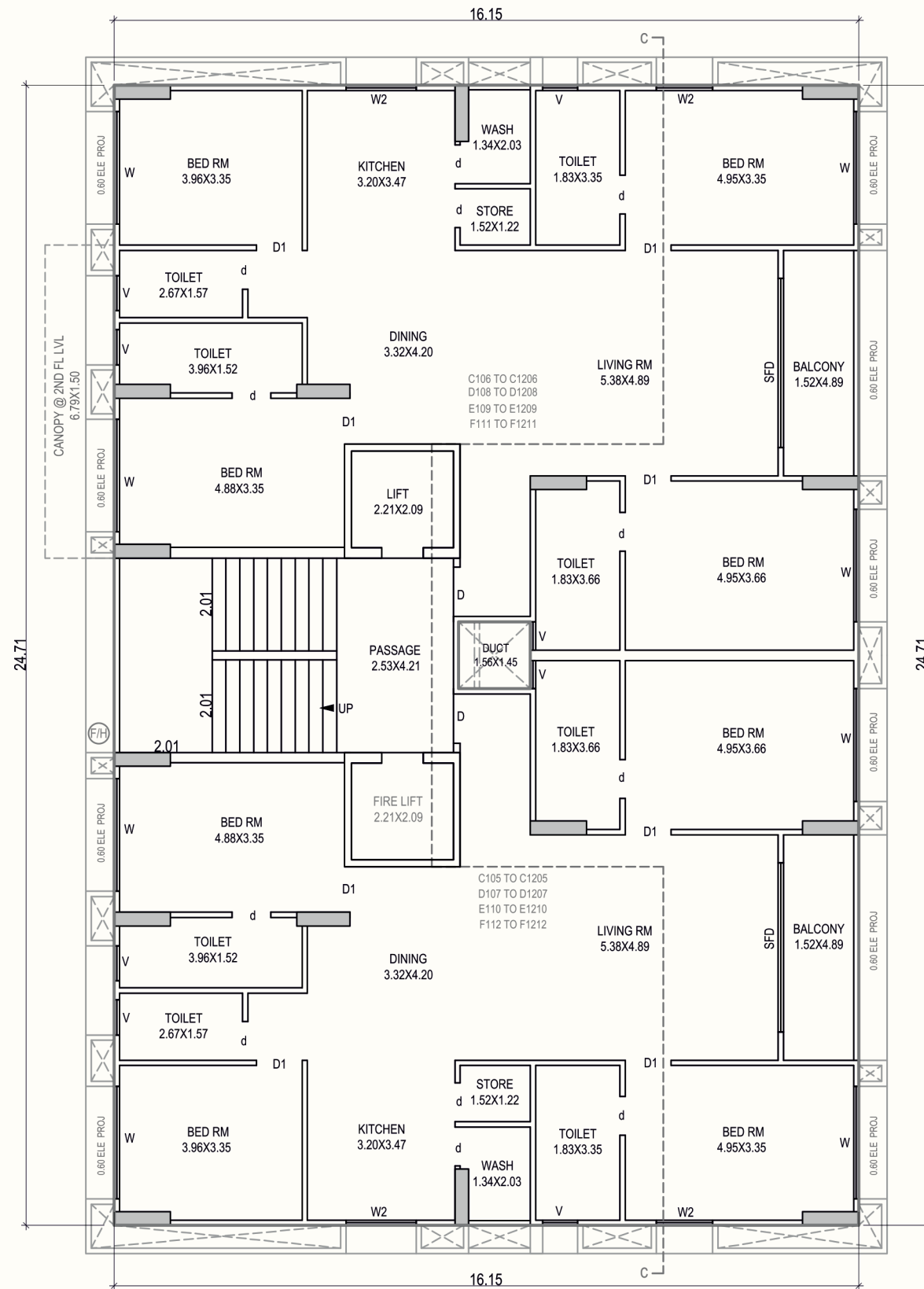
C-D-E-F BUILDING 1ST -12TH FLOOR PLAN
