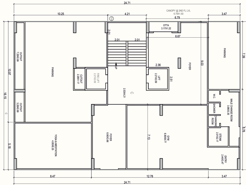
C-BUILDING GROUND FLOOR PLAN
