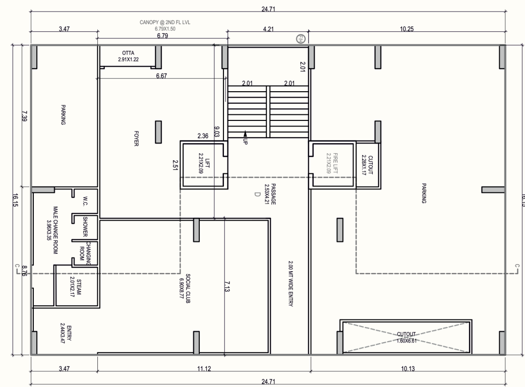
D-BUILDING GROUND FLOOR PLAN
