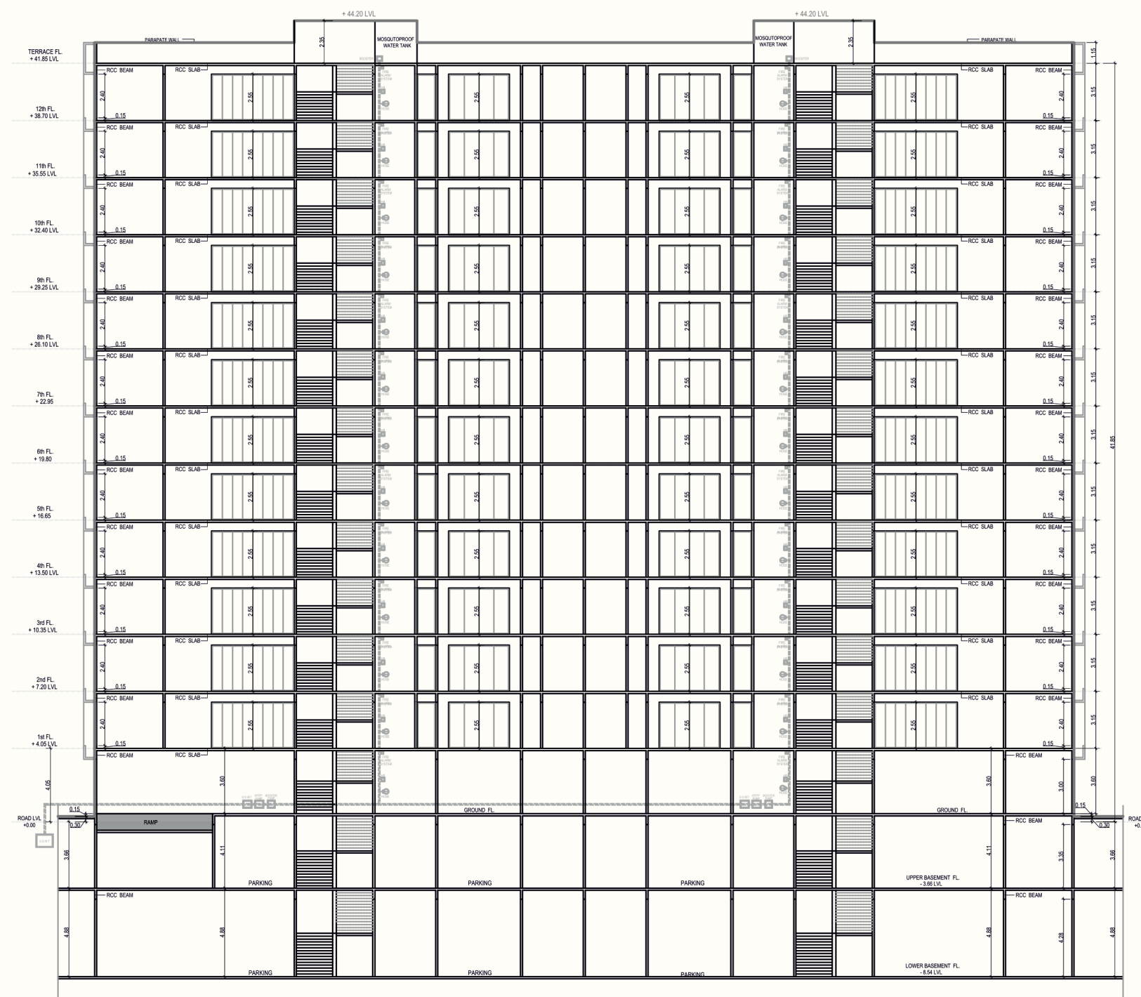
A-B BUILDING SECTION
