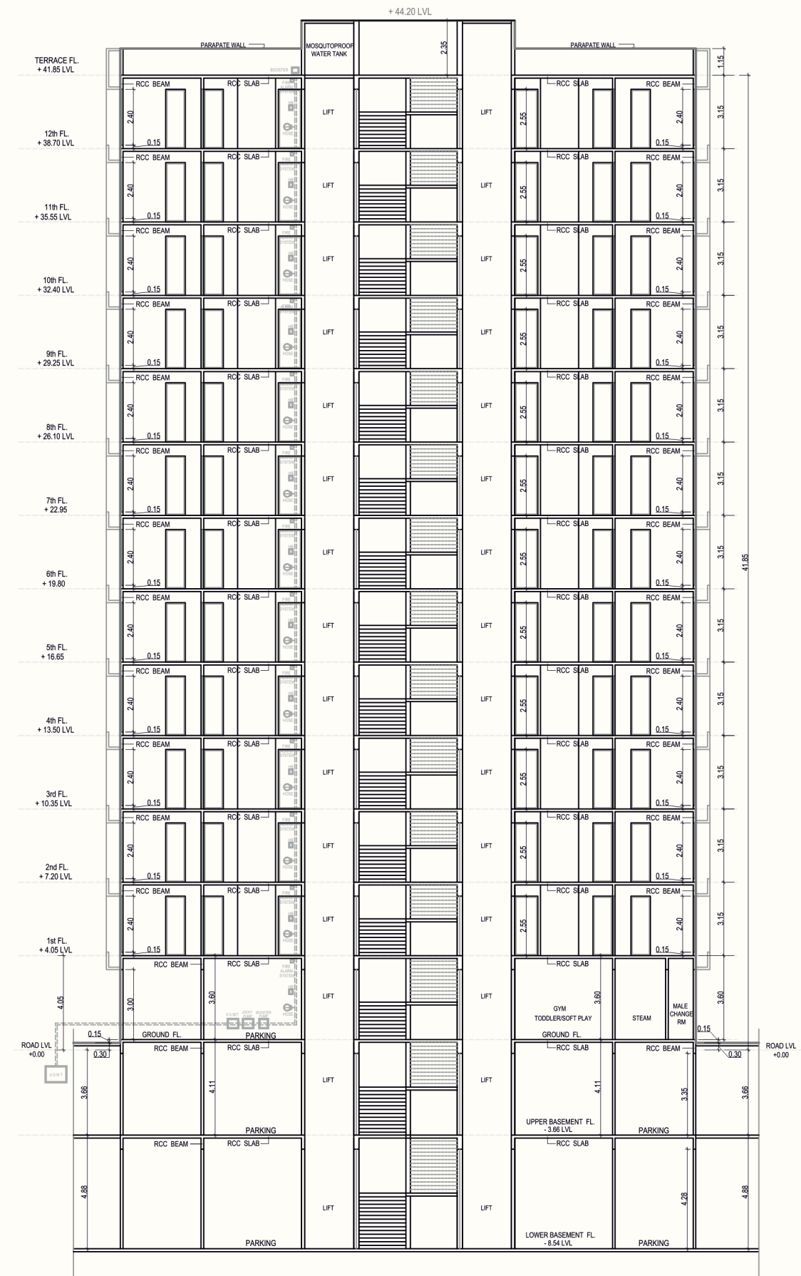
C-D-E-F BUILDING SECTION
