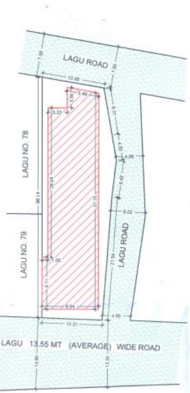
LAYOUT PLAN SCALE: 1/10M = 4.00 MT.
